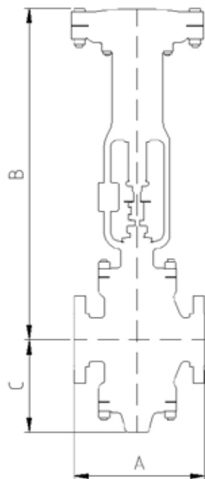
R6571—R6574 结构尺寸图 /R6571—R6574 flanged valve dimensional drawing
