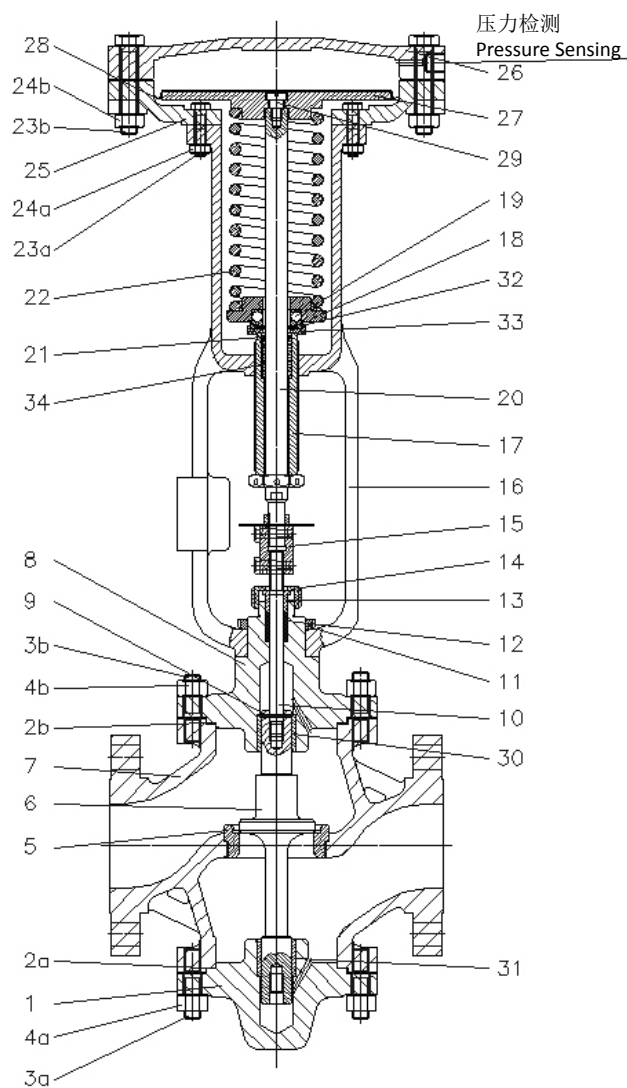
R6581, R6582 剖面图 /Sectional Drawings
