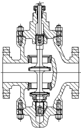
R6573, R6574 剖面图 /Sectional Drawings
