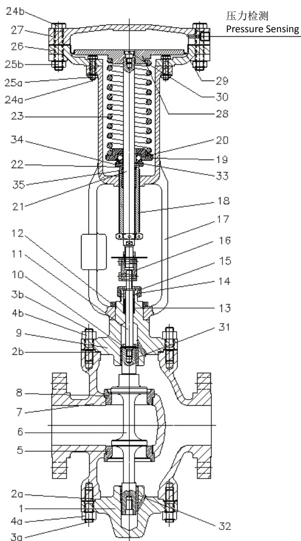
R6571, R6572 剖面图 / Sectional Drawings
