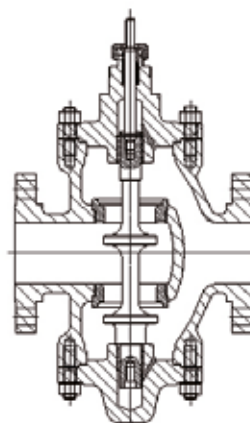
R6571, R6572 剖面图 / Sectional Drawings
