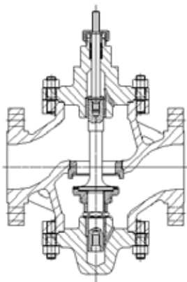
R6583, R6584 剖面图 /Sectional Drawings
