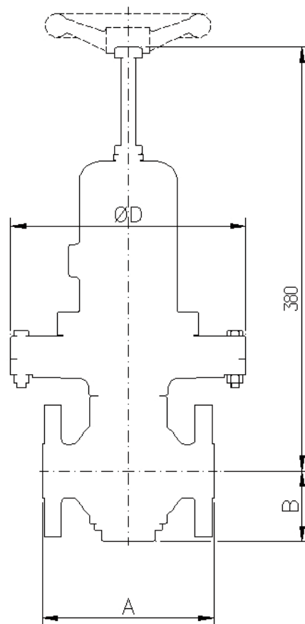
阀体尺寸和端面距离 / Body sizes and face to face dimensions
