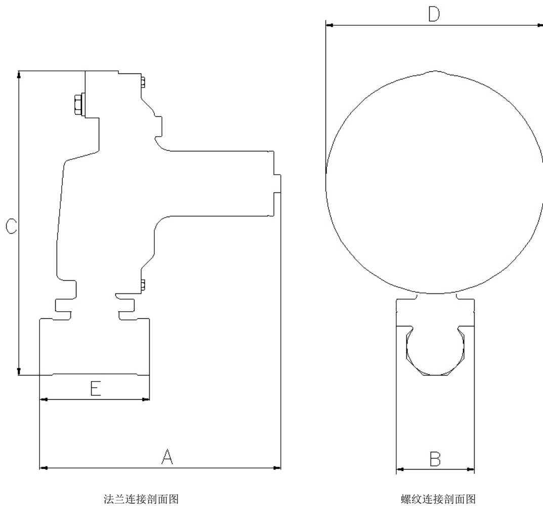
阀体尺寸和端面距离 / Body sizes and face to face dimensions
