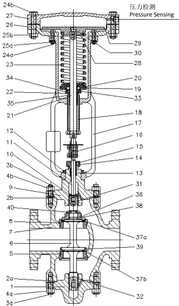
R6573, R6574 剖面图 /Sectional Drawings
