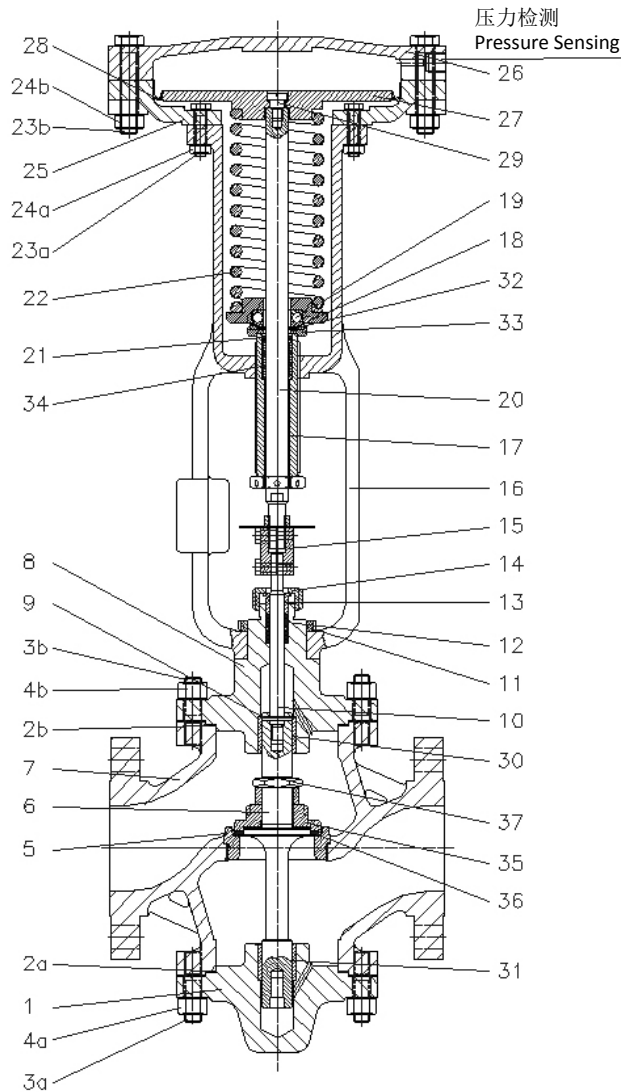
R6583, R6584 剖面图 /Sectional Drawings
