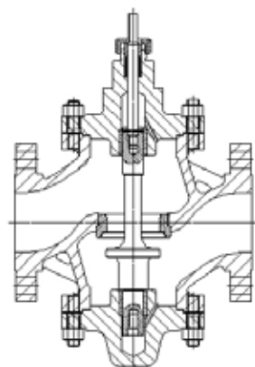
R6581, R6582 剖面图 /Sectional Drawings
